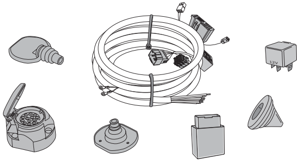
CV621ADE01PC
